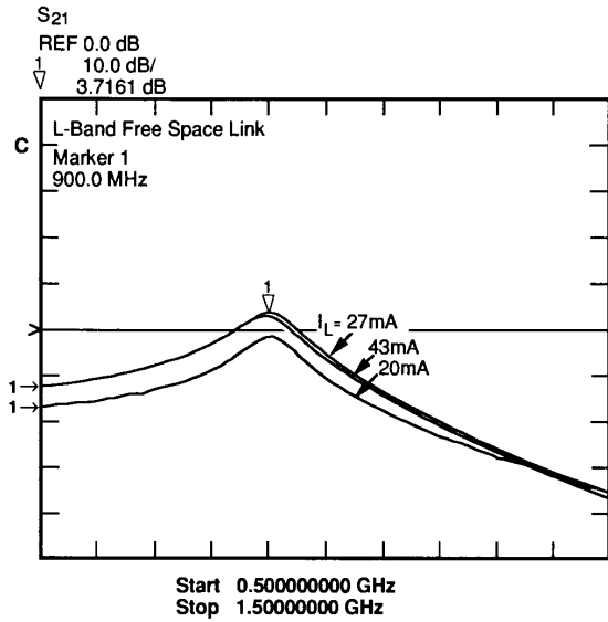
Figure 2. Measured insertion gain of L-band optical link under various laser diode biasing conditions.
